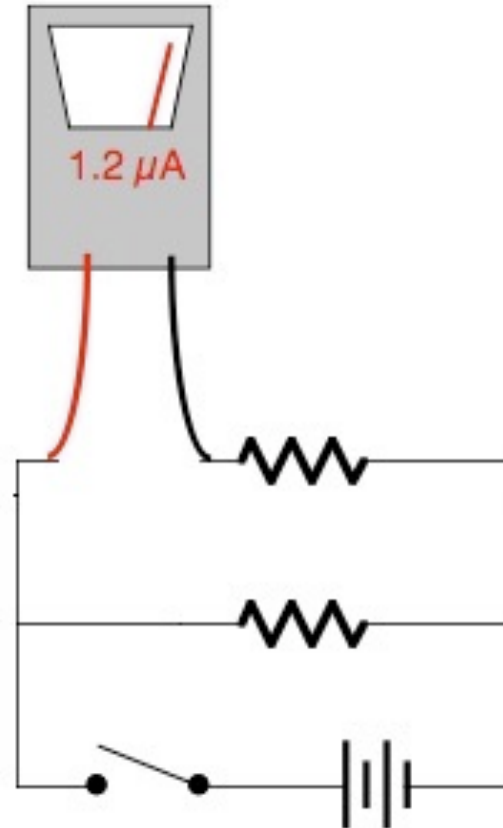
Measuring current
